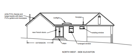
NORTH WEST - SIDE ELEVATION
